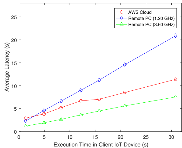
Fig. 2. Effect of application's execution time in client IoT device on average latency (Boltzmann machine).
